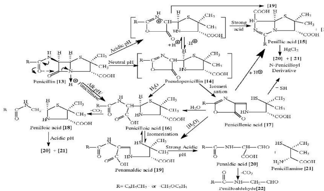
Figure 4. Pathways of degradation of penicillin in acidic and alkaline conditions.
